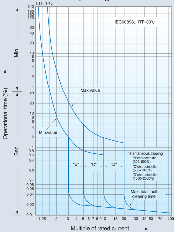
Operating curves
